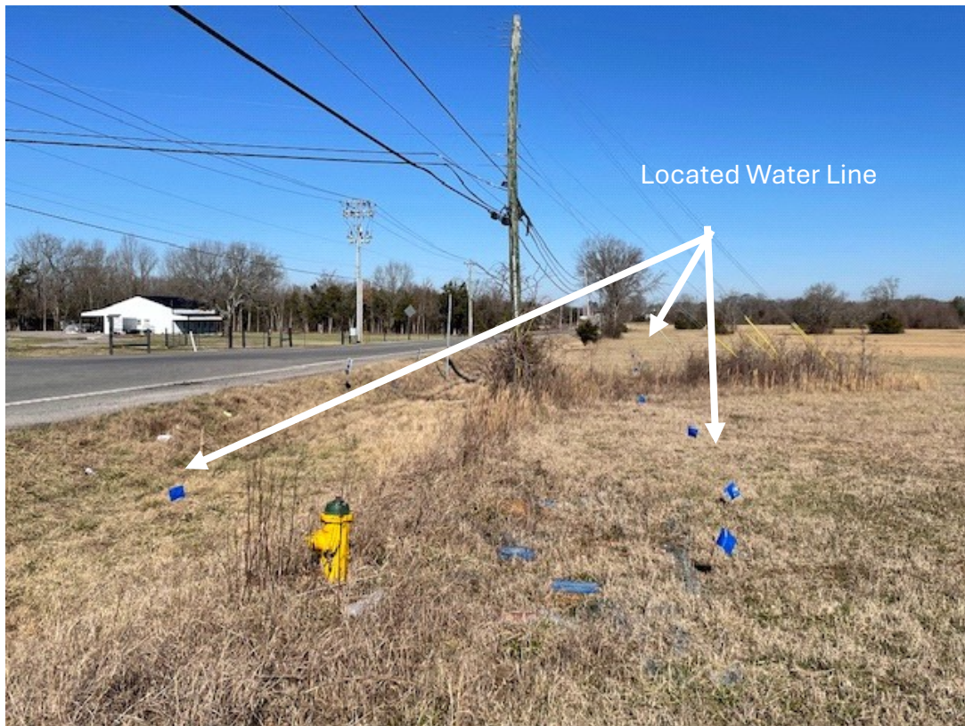
Water Lines – Manchester Pike at Epps Mill intersection facing north
