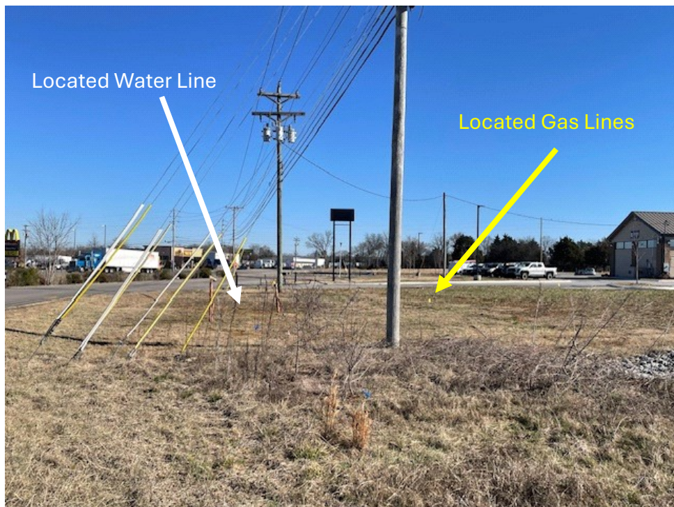
Power, Water, and Gas Lines – Miller Ln facing northeast (Power and water adjacent to Miller; gas line crosses under)
